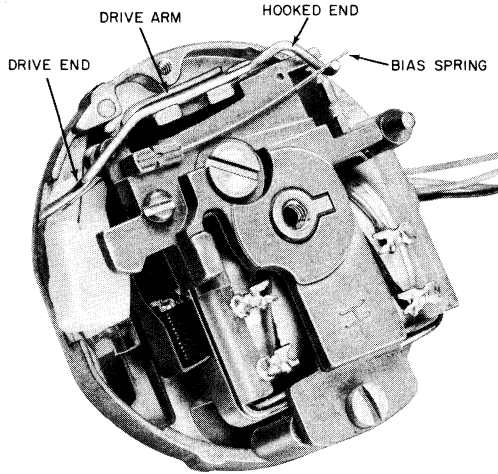
Fig. 7—Cover Removed to Show Drive Arm and Bias Spring
