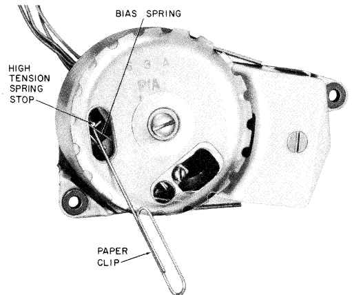
Fig. 6—Positioning Bias Spring
