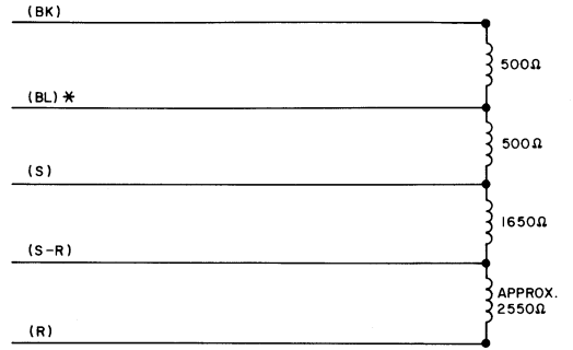
A. PIA AND P3A RINGER
