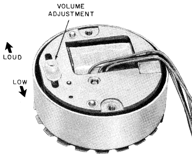
Fig. 4—P-Type Ringer (Bottom View)
